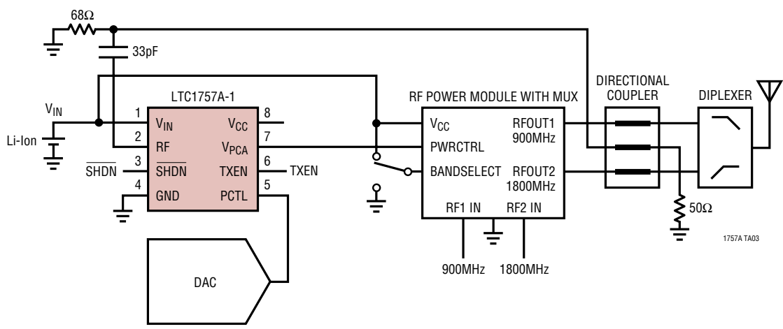
Using the LTC1757A-1 in a Dual Band Cellular Telephone Transmitter Without Current Limiting
