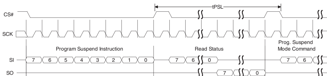
Figure 10.59 Program Suspend Command Sequence
