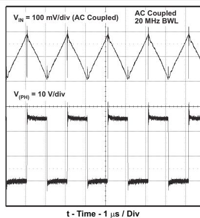
Figure 7-5. Input Voltage Ripple and PH Node, I_O = 1\text{ A}
