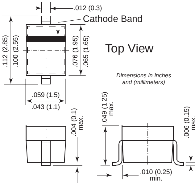
SOD-323
