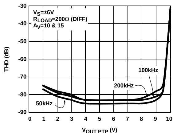
FIGURE 10. DISTORTION RESULTS
