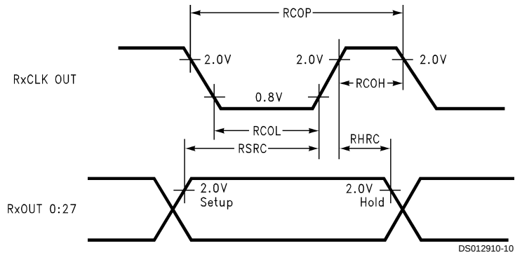
FIGURE 7. DS90CR286 (Receiver) Setup/Hold and High/Low Times
