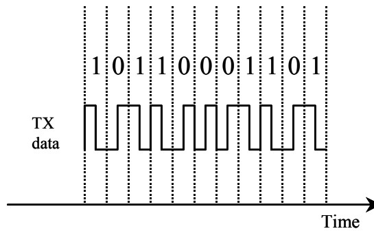
Figure 10. Manchester encoding
