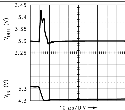
Figure 25. Line Transient Response ( I_{OUT} = 800 \text{ mA} )
