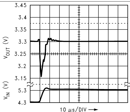
Figure 24. Line Transient Response ( I_{OUT} = 800 \text{ mA} )
