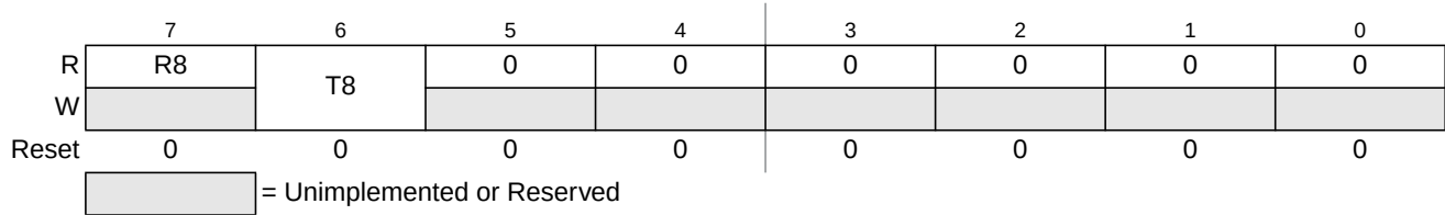
Figure 11-12. SCI Data Registers (SCIDRH)
