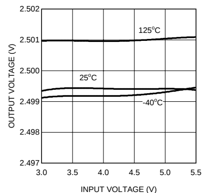
Figure 50. Line Regulation
