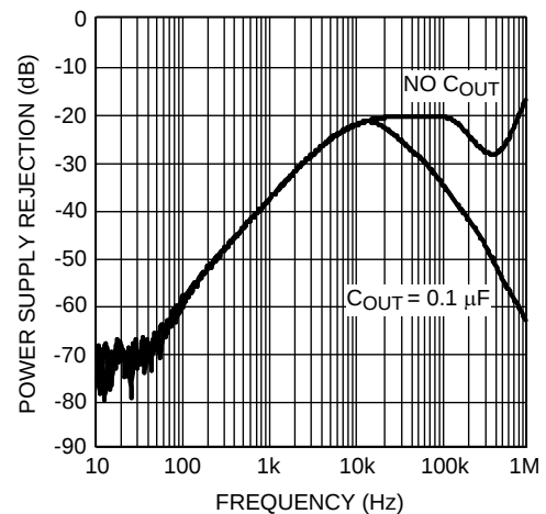
Figure 40. Power Supply Rejection vs Frequency
