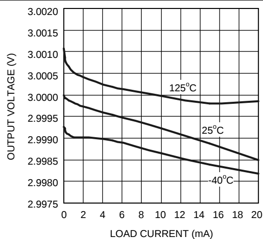
Figure 30. Load Regulation
