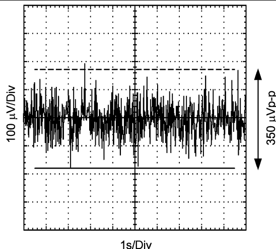
Figure 44. 0.1–10 Hz Noise
