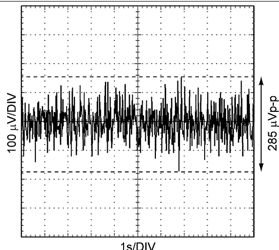
Figure 32. 0.1–10 Hz Noise
