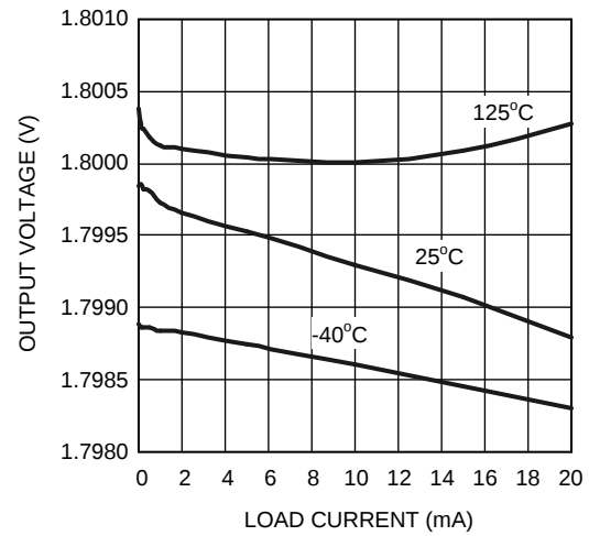
Figure 12. Load Regulation
