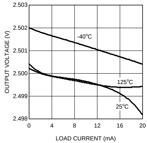
Figure 24. Load Regulation
