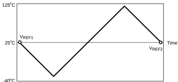
Figure 47. Temperature Profile
