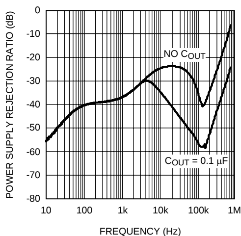
Figure 46. Power Supply Rejection vs Frequency
