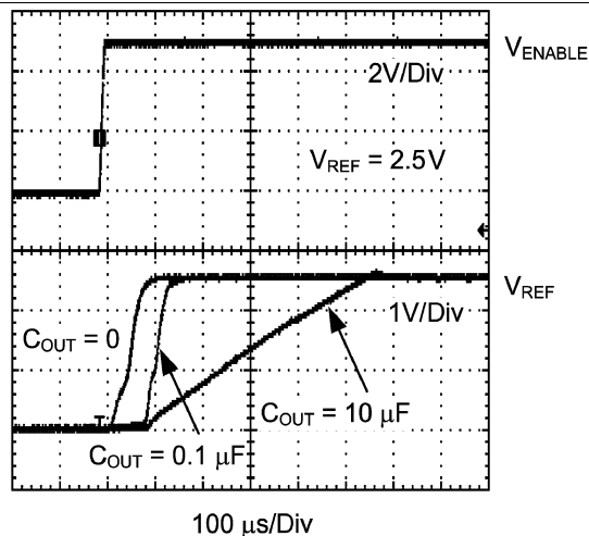
Figure 8. Turnon Transient Response
