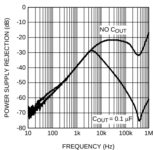
Figure 34. Power Supply Rejection vs Frequency
