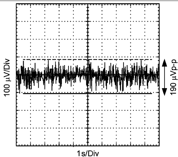
Figure 20. 0.1–10 Hz Noise
