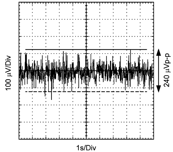
Figure 26. 0.1–10 Hz Noise
