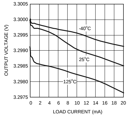
Figure 36. Load Regulation
