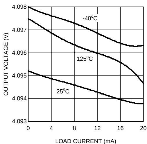
Figure 42. Load Regulation
