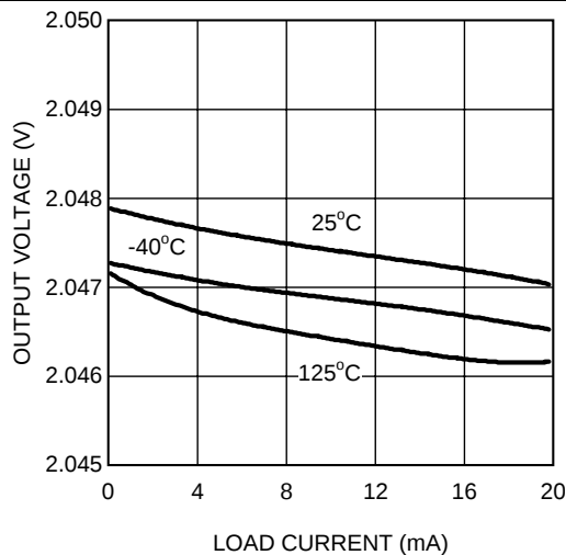
Figure 18. Load Regulation
