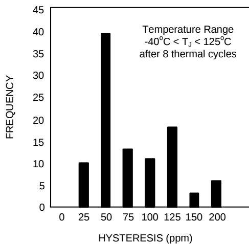
Figure 7. Typical Thermal Hysteresis
