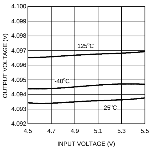
Figure 43. Line Regulation
