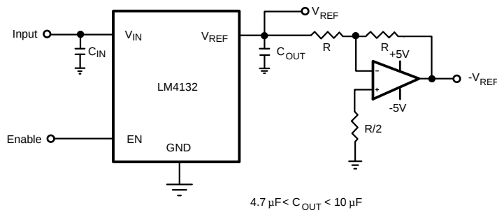
Figure 51. Voltage Reference With Complementary Output
