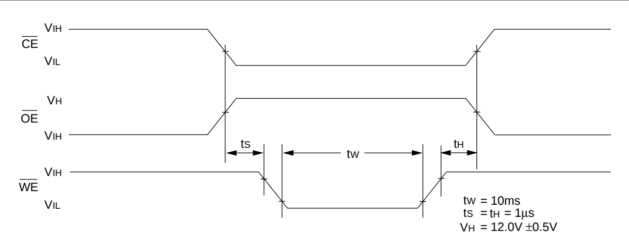
FIGURE 1-4: CHIP CLEAR WAVEFORMS
