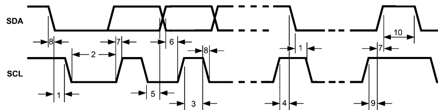
Figure 1. I 2 C-Compatible Timing
