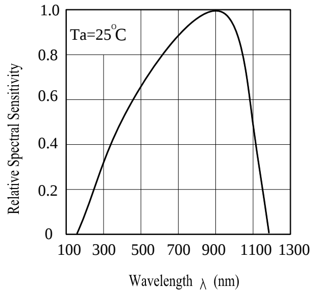
Spectral Sensitivity
