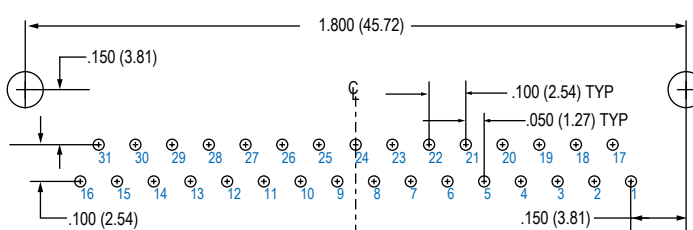
31 PIN
