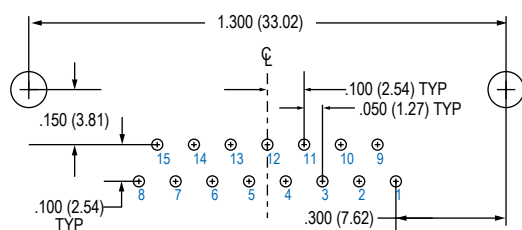
15 PIN
