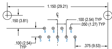
9 PIN
