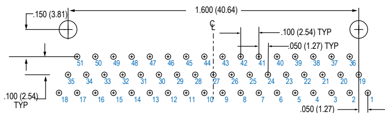
51 PIN
