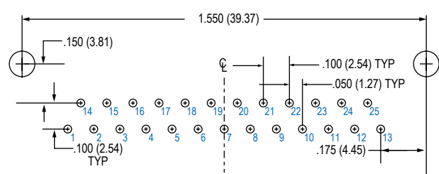
25 SOCKET
