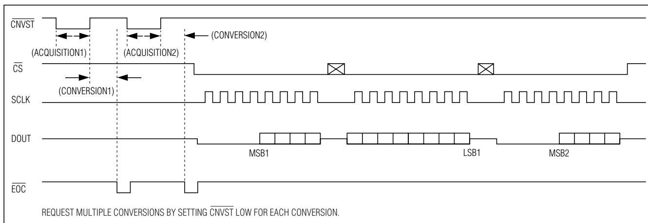
Figure 5. Clock Mode 01
