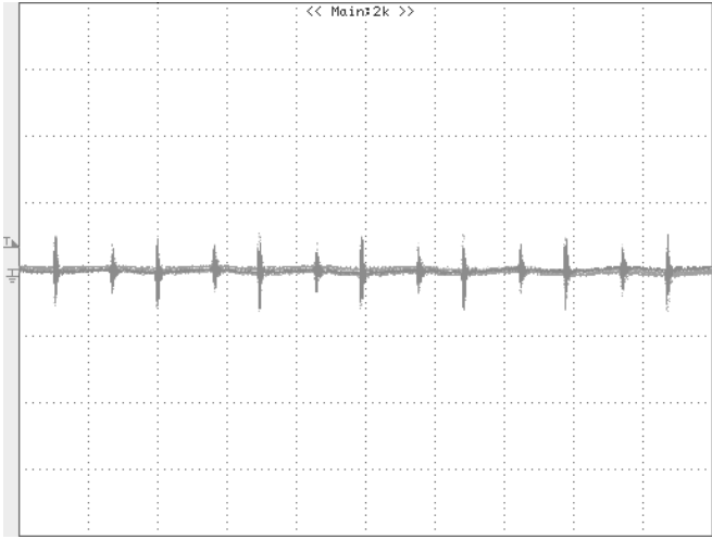
Figure 12: Input reflected ripple current, i_s , through a 12\mu\text{H} source inductor at nominal input voltage and rated load current (50 mA/div, 2µs/div)
