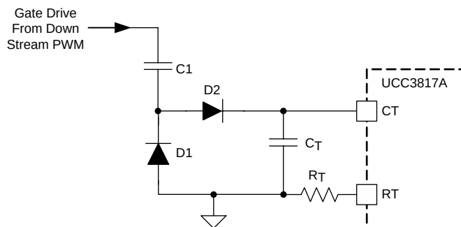
Figure 11. Synchronizing the UCC3817A to a Down-Stream Converter
