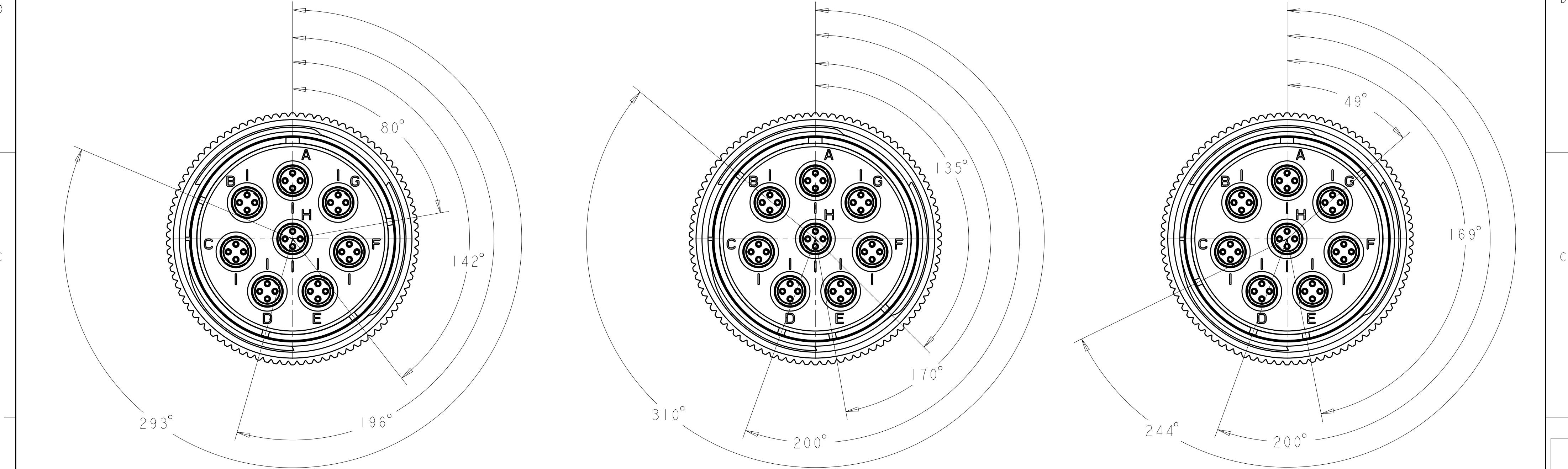
1811928-1 "N" KEY POLARIZATION
