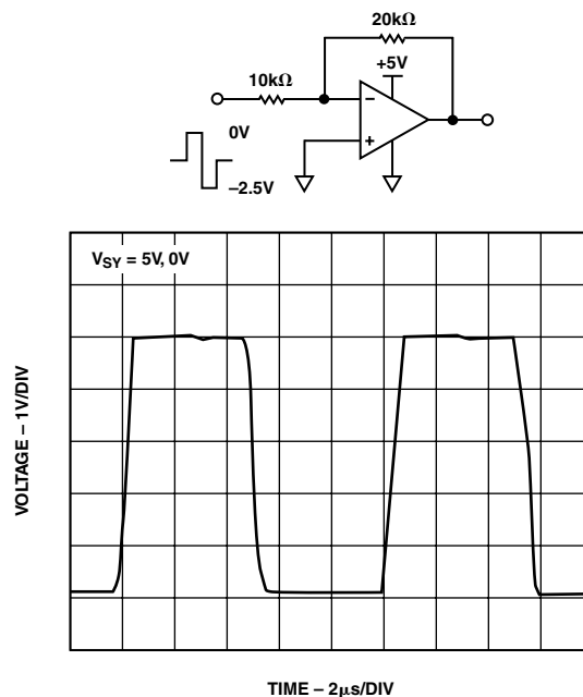
Figure 2a. Gain of Two Inverter Response to 2.5 V Step, Centered -1.25 V Below Ground
