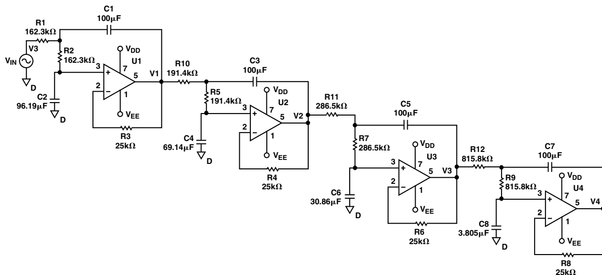
Figure 7. 10 Hz, Eight-Pole Sallen Key Low-Pass Filter
