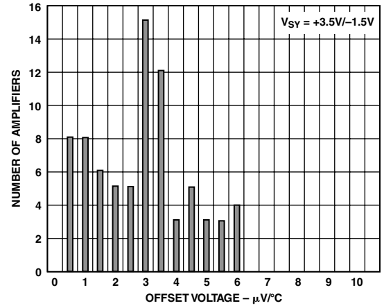
TPC 4. Offset Voltage Drift
