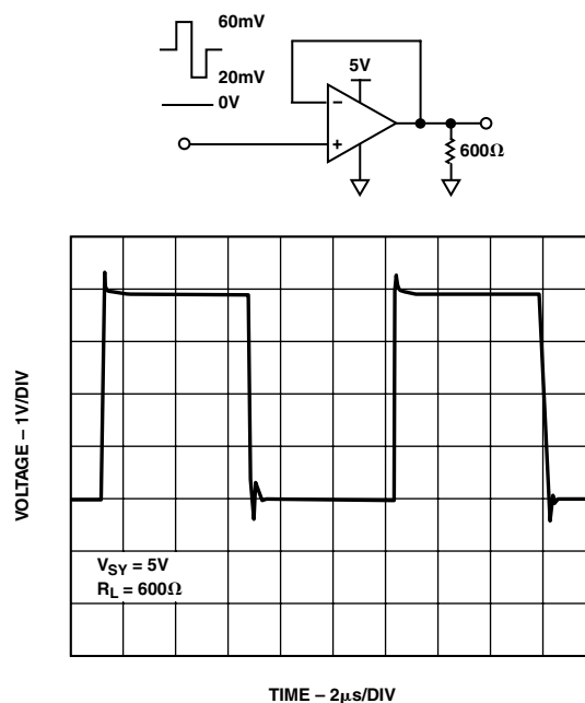
Figure 2b. Unity Gain Follower Response to 40 mV Step, Centered 40 mV Above Ground
