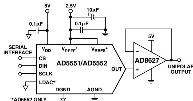
Figure 5. Unipolar Output
