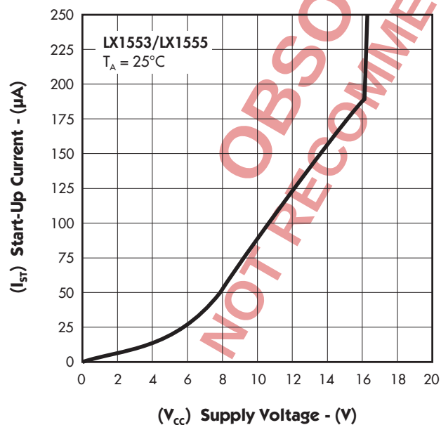
FIGURE 11. — START-UP CURRENT vs. SUPPLY VOLTAGE
