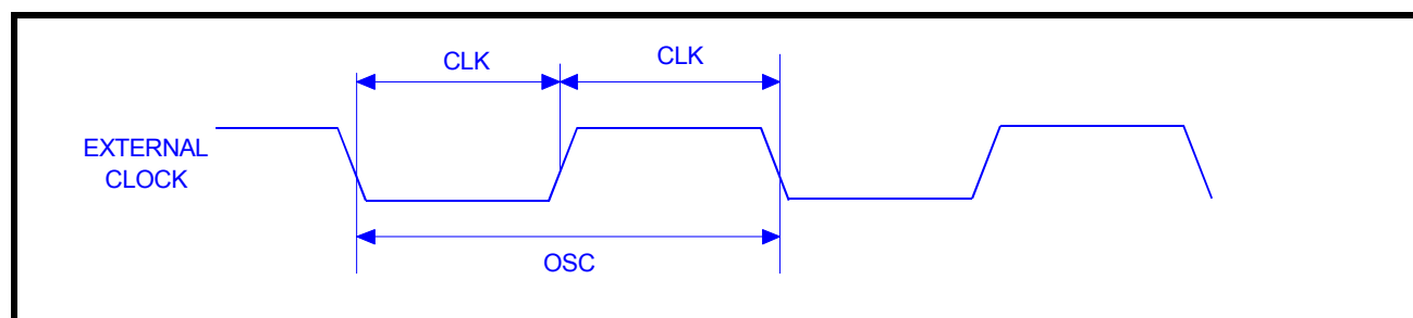
FIGURE 21. CLOCK TIMING
