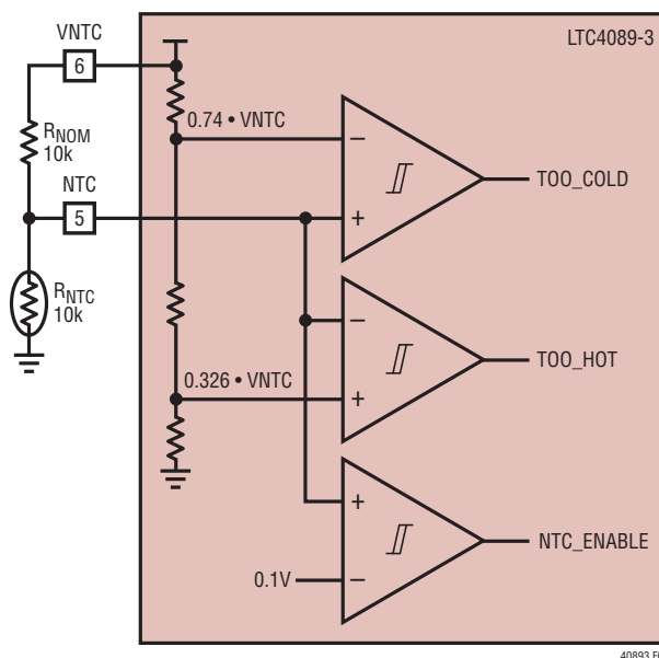
Figure 4. NTC Circuit
