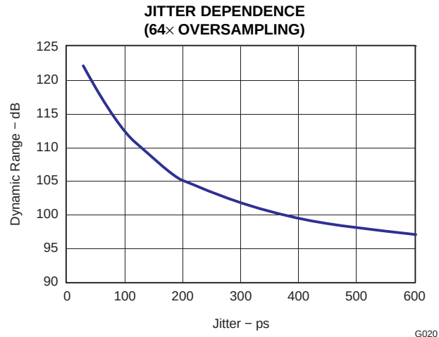
Figure 38. Jitter Sensitivity
