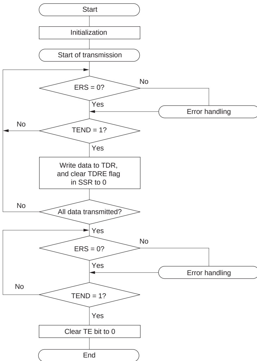
Figure 13.4 Sample Transmission Flowchart
