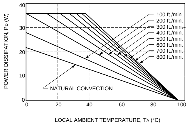
Figure 12. Power Derating vs. Local Ambient Temperature and Air Velocity
