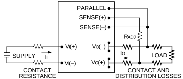
Figure 6. Circuit Configuration to Adjust Output Voltage.
