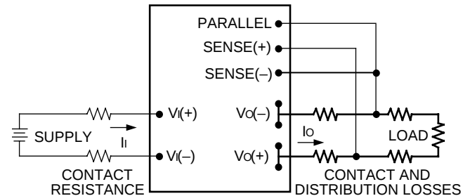
Figure 3. Effective Circuit Configuration for Single-Module Remote Sense Operation
