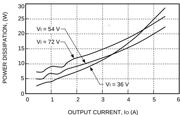
Figure 10. Power Dissipation as Heat vs. Output Current
