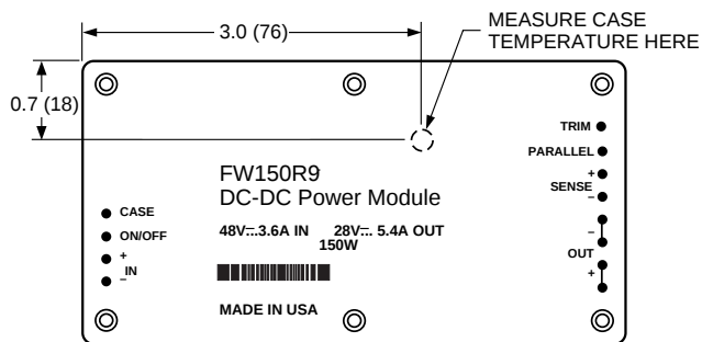
Figure 9. Case Temperature Measurement Location
