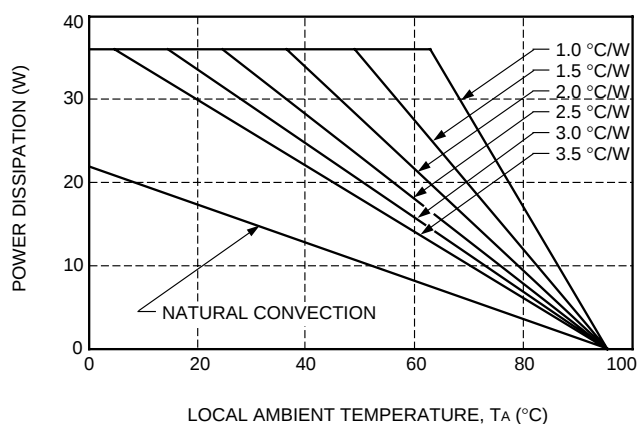
Figure 11. Power Derating vs. Local Ambient Temperature and Heat Sink Resistance
