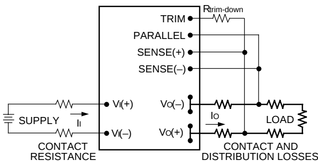
Figure 5. Circuit Configuration to Trim Down Output Voltage
