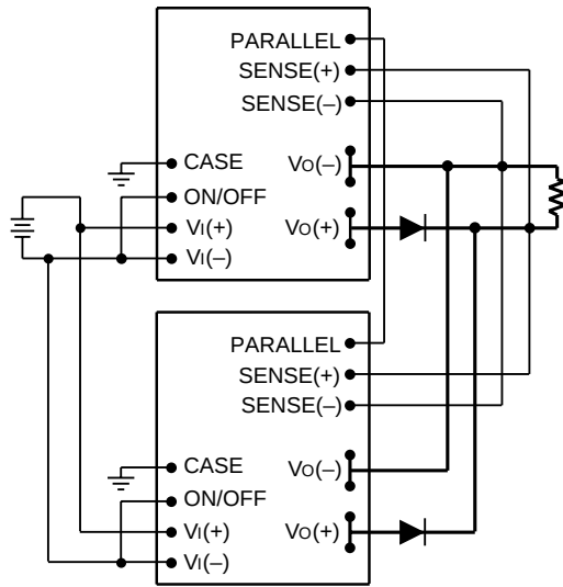
Figure 7. Wiring Configuration for Redundant Parallel Operation
