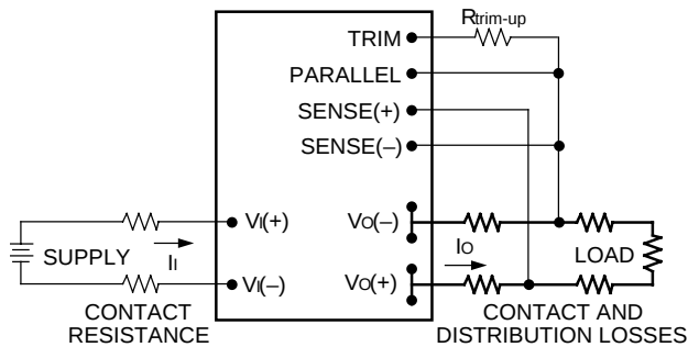
Figure 4. Circuit Configuration to Trim Up Output Voltage
