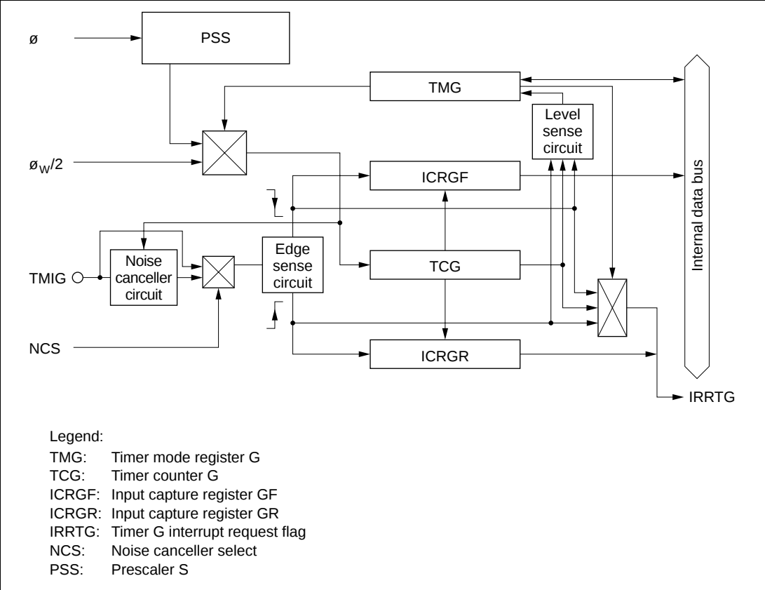
Figure 9.6 Block Diagram of Timer G
