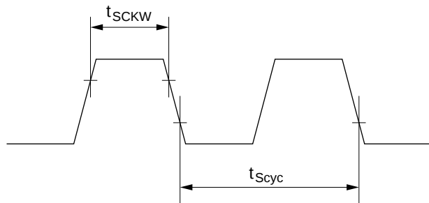
Figure 14.5 SCK 3 Input Clock Timing
