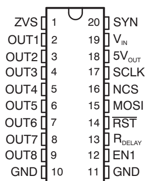
N OR PWP PACKAGE (TOP VIEW)
