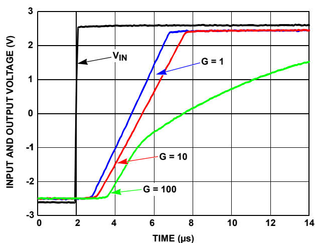
FIGURE 51. NEGATIVE OVERLOAD RECOVERY TIME, ISL2853x
