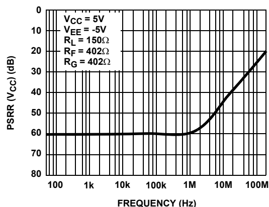
FIGURE 11. PSRR +5V
