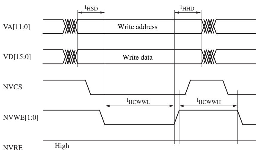
Figure 7. Host memory and register write timing
