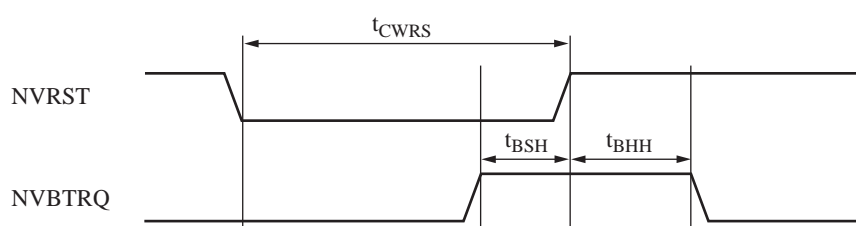
Figure 11. Reset and boot timing
