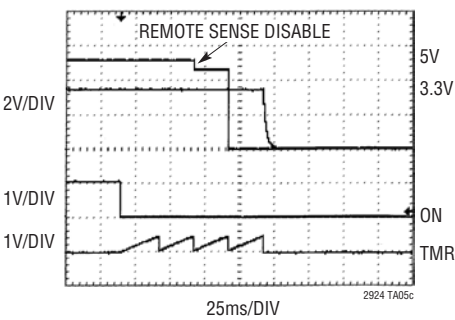
Power-Off
