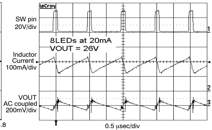
Figure 9. Switching Waveforms
