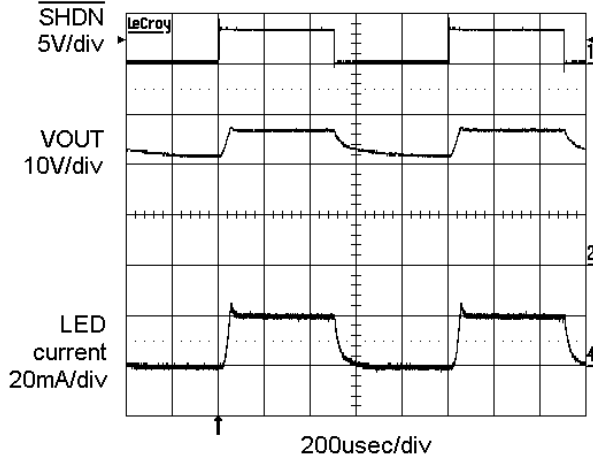
Figure 25. Switching Waveform with 1 kHz PWM on \overline{\text{SHDN}}
