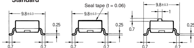
Flat Actuator Standard
