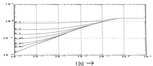
Transient Thermal impedance Z_{th(jh-c)} = f(t) parameter: D = 1/T
