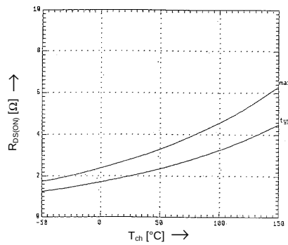
Drain-Source On-State Resistance R_{DS(on)} = f(T_{ch}) ; I_D = 5\text{A} ; V_{GS} = 10\text{V}
