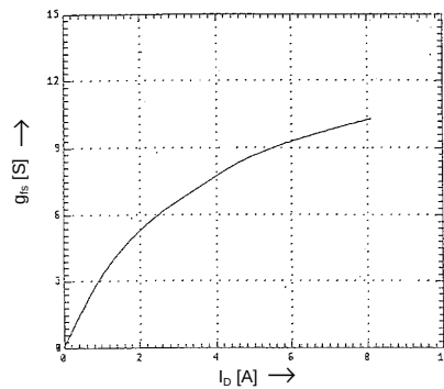
Typical Forward Transconductance g_{fs} = f(I_D) ; 80μs pulse test; V_{DS} = 25\text{V} ; T_{ch} = 25^\circ\text{C}
