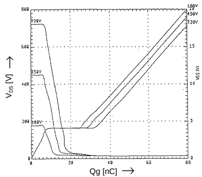
Typical Gate Charge Characteristics V_{GS} = f(Q_g) ; I_D = 5\text{A}
