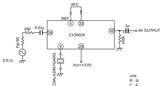
Test Circuit
