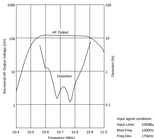
Frequency Characteristics
