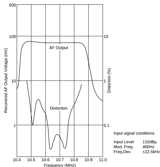
Frequency Characteristics
