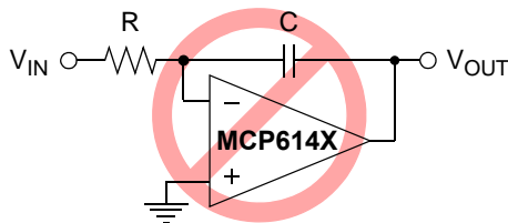
FIGURE 4-5: Examples of Unstable Circuits for the MCP6141/2/3/4 Family.
