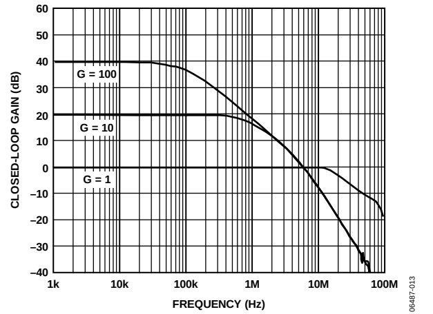
Figure 13. Closed-Loop Gain vs. Frequency
