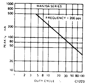
Fig. 15. Max Peak Current vs. Duty Cycle
