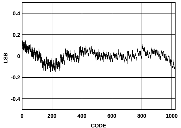
FIGURE 18. INTEGRAL NONLINEARITY
