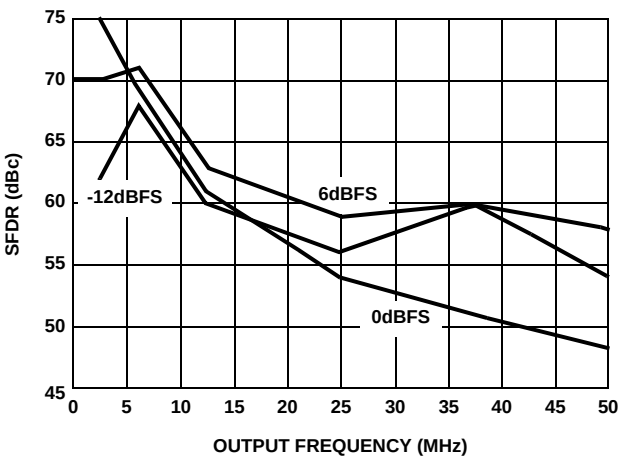
FIGURE 5. SFDR vs f_{OUT} , CLOCK = 125MSPS
