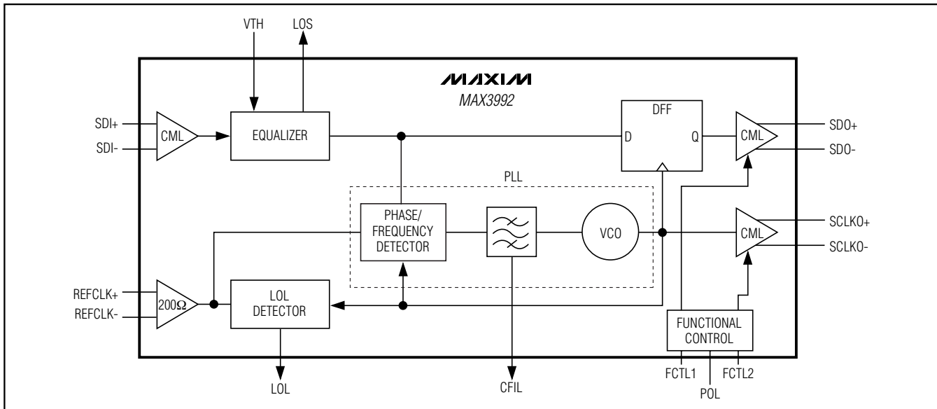
Figure 3. Functional Diagram
