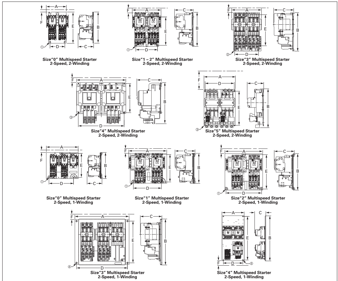
Figure 33-39. Approximate Dimensions
