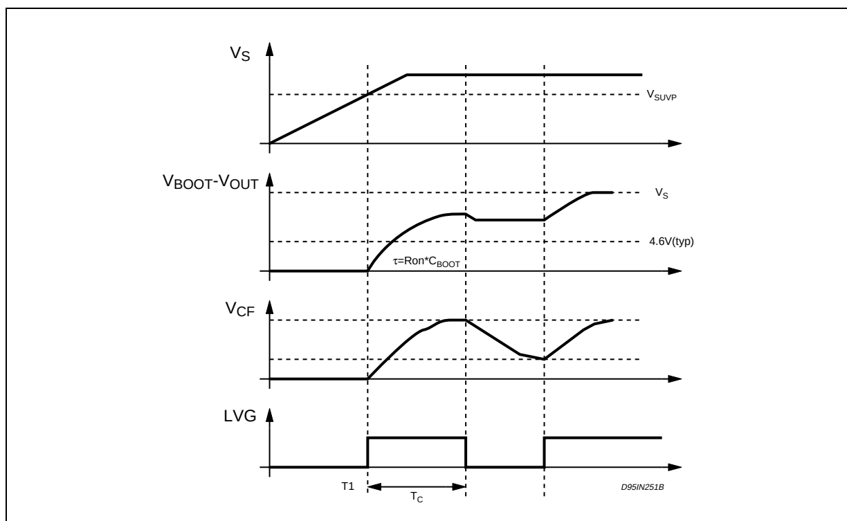
Figure 3. Waveforms (L6569A)
