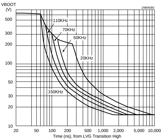
Figure 8. V_{boot} pin SOA @ T_j = 125^\circ\text{C}
