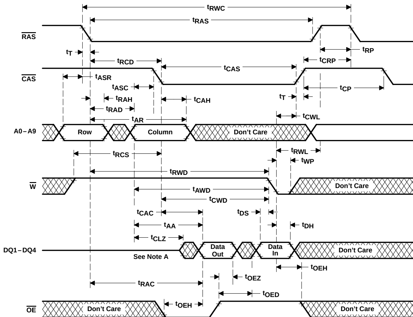
Figure 7. Read-Write-Cycle Timing
