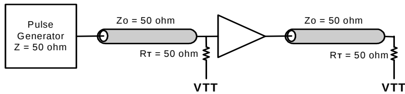
Figure 1. AC Test Reference for V_{DD} = 3.3V / 2.5V
