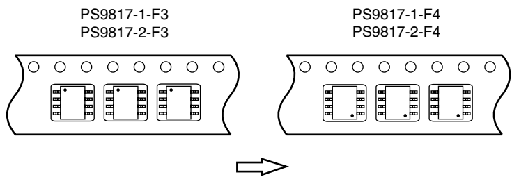
Taping Direction
