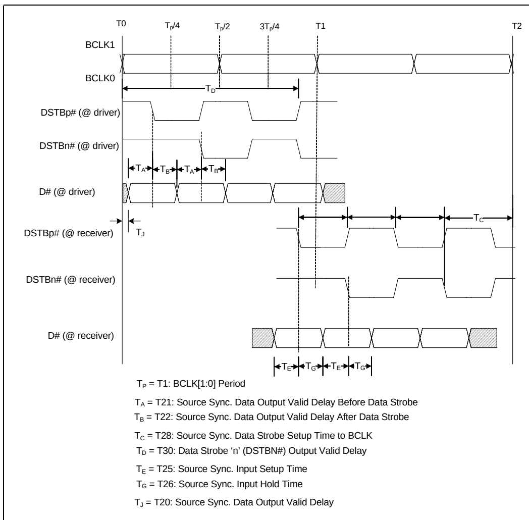
Figure 2-18. FSB Source Synchronous 4X (Data) Timing Waveform
