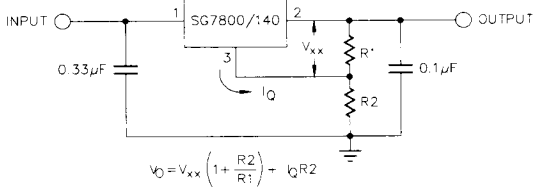
FIGURE 6 - CIRCUIT FOR INCREASING OUTPUT VOLTAGE
