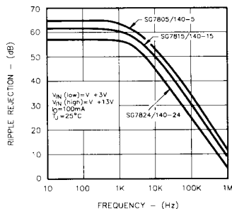
FIGURE 3. RIPPLE REJECTION VS. FREQUENCY
