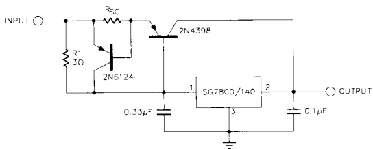
FIGURE 7 - HIGH OUTPUT CURRENT, SHORT CIRCUIT PROTECTED
