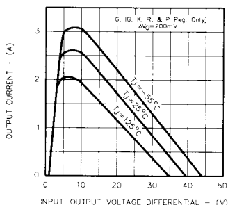
FIGURE 1. PEAK OUTPUT CURRENT VS. INPUT - OUTPUT DIFFERENTIAL
