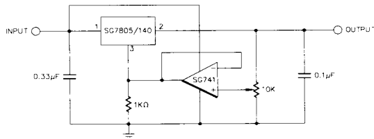
FIGURE 8 - ADJUSTABLE OUTPUT REGULATOR, 7V TO 30V
