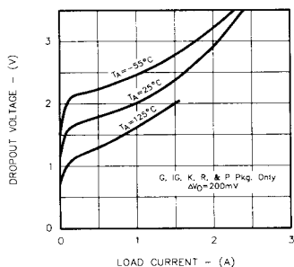
FIGURE 2. MINIMUM INPUT - OUTPUT VOLTAGE VS. LOAD CURRENT
