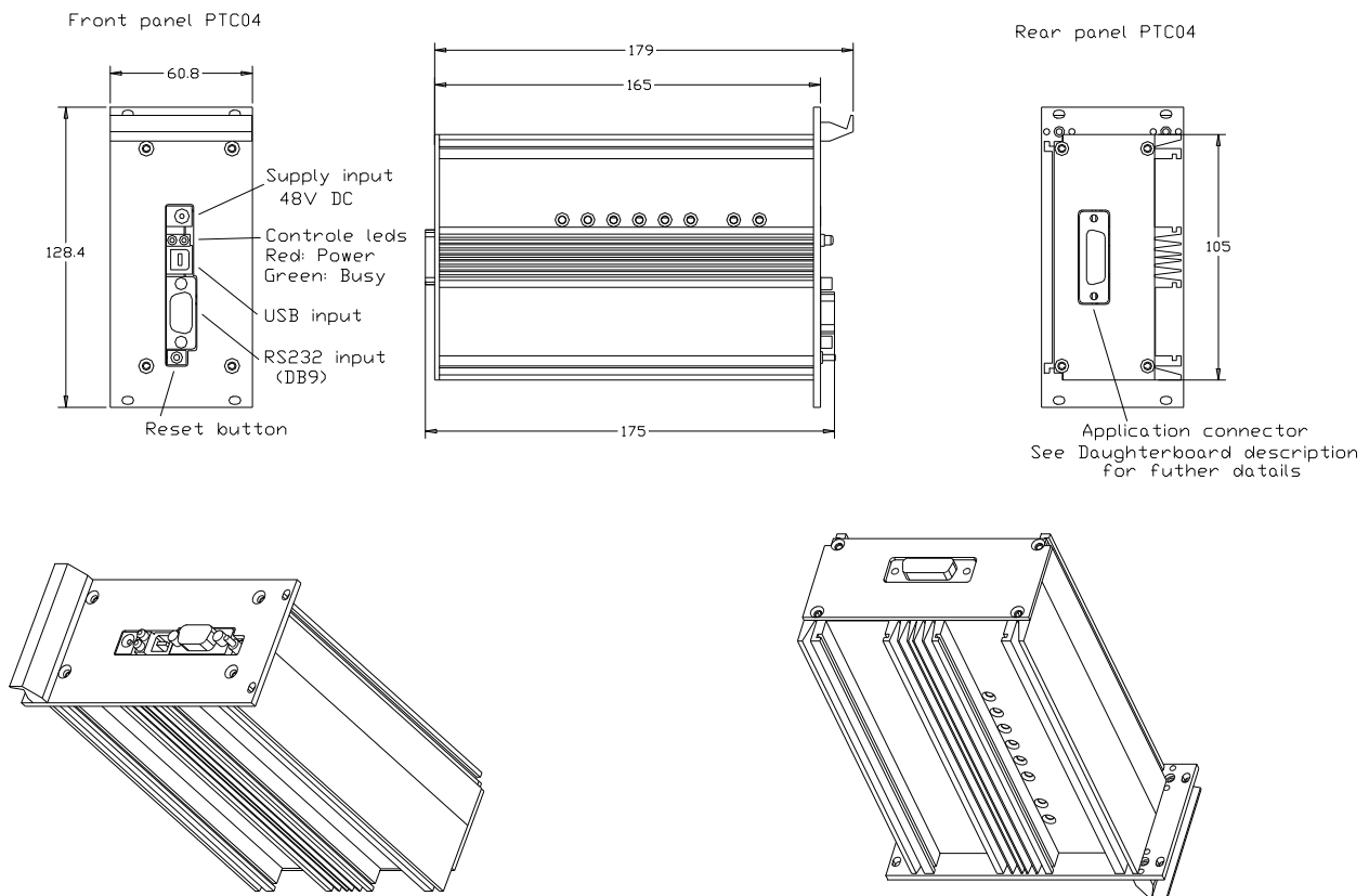
Figure 21-1: Mechanical Outlines
