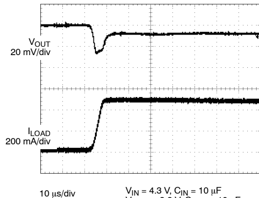
Load Transient Response-5
