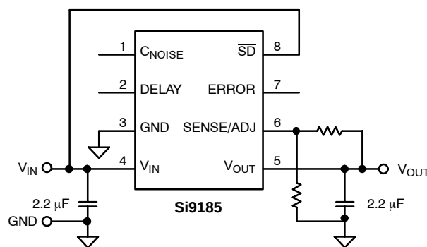
FIGURE 2. Adjustable Output
