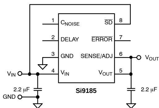
FIGURE 1. Fixed Output
