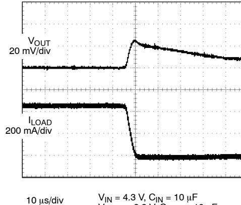
Load Transient Response-6
