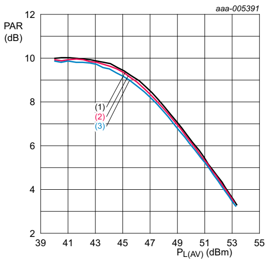
V_{DS} = 28\text{ V}; I_{Dq} = 2400\text{ mA}. (1) f = 2110\text{ MHz} (2) f = 2140\text{ MHz} (3) f = 2170\text{ MHz}
